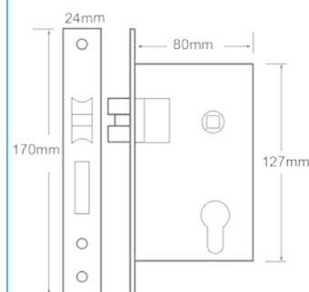
Latch bolt & dead bolt
