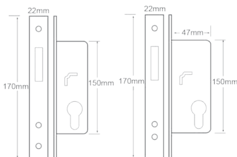
Hook Lock
